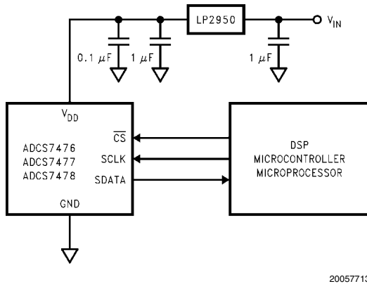
FIGURE 8. Typical Application Circuit
